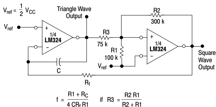
Figure 16. Function Generator
