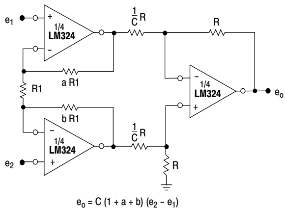
Figure 13. High Impedance Differential Amplifier
