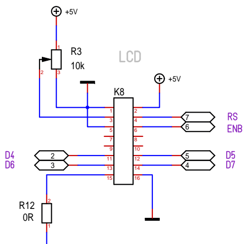
MC41605B6W-SPTLY LiquidCrystal lcd(7,6,2,5,3,4);
