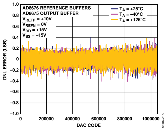
Figure 12. Differential Nonlinearity Error vs. DAC Code, \pm 10 V Span, X2 Gain Mode
