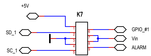
SUB-D-9-STIFT-ST
