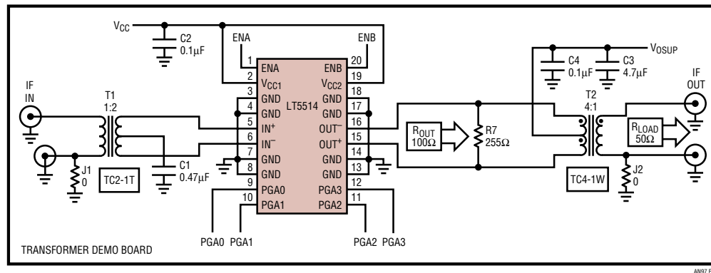
Figure 3. Output Transformer Application Board (Simplified Schematic)
