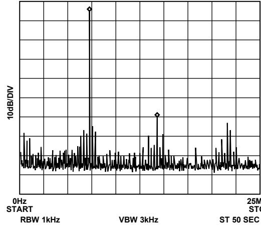
Figure 16. f_{MCLK} = 50 MHz, f_{OUT} = 7.1 MHz. Frequency Word = 245AICAC
