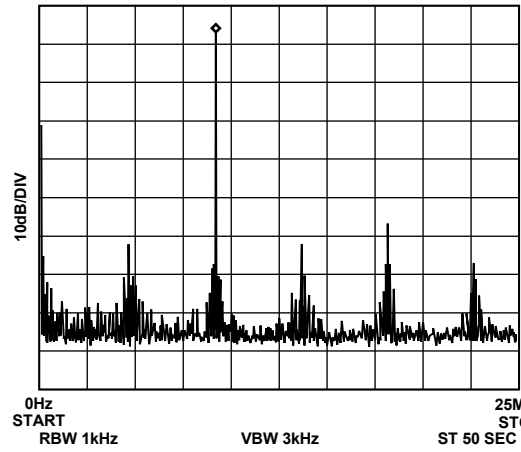
Figure 17. f_{MCLK} = 50 MHz, f_{OUT} = 9.1 MHz. Frequency Word = 2E978D50
