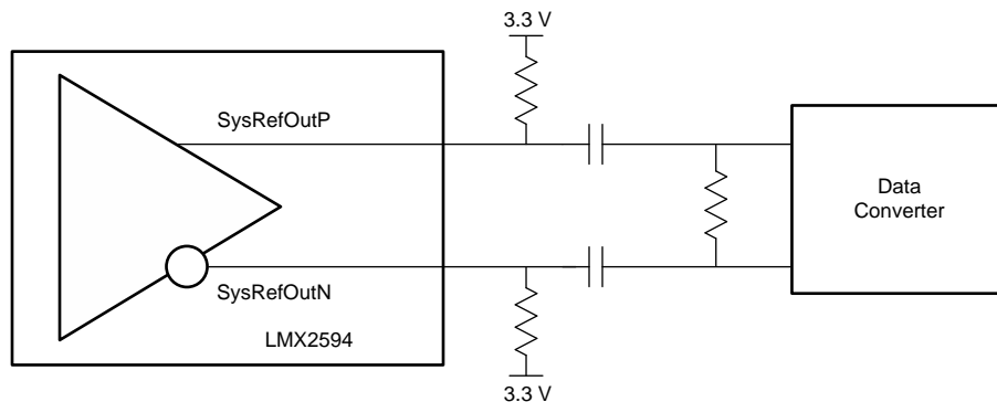
Figure 32. SYSREF Output
